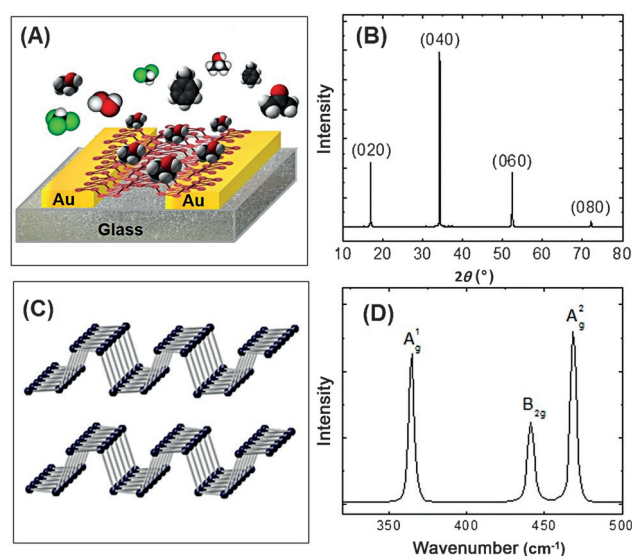
Figure 1. a) Vapor sensor based on black phosphorus. b) X-ray diffractogram of black phosphorus. c) The crystalline structure of black phosphorus. d) Raman spectrum of black phosphorus.
